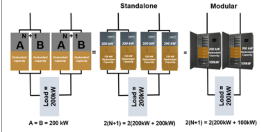
Figure 5: Redundancy at both UPS and power distribution path level
